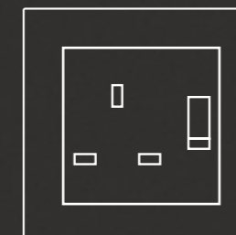
British Standard 13 A, switchable
